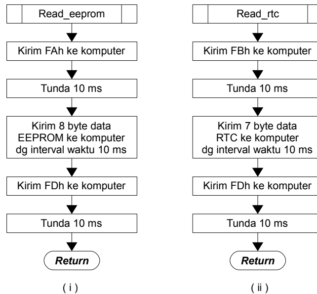
Gambar 3 Flowchart Sub Rutin Read_eeprom dan Read_rtc
